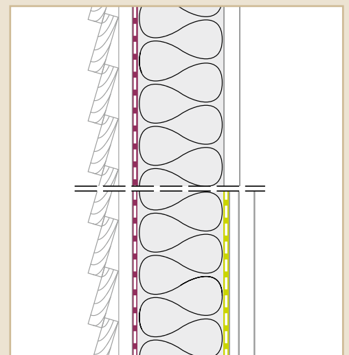
External wall wrap 2.50 MNs/g (medium vapour resistance)
