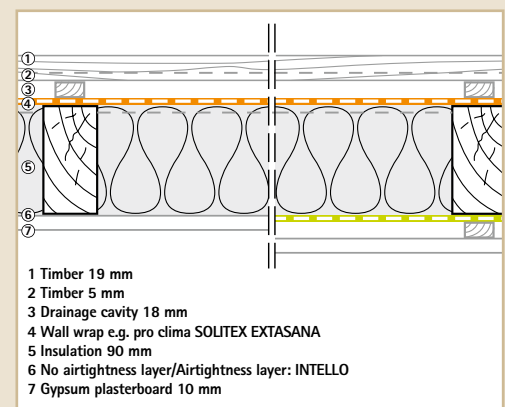
Fig. 35. Wall construction B
