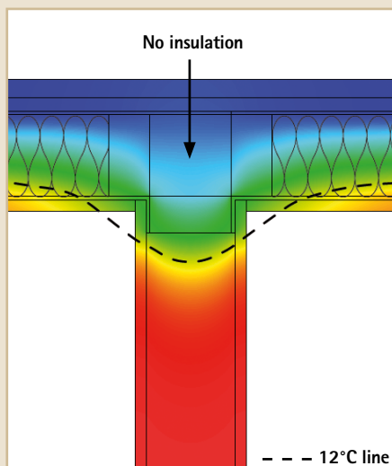
Uninsulated joints of integrated internal walls cause thermal bridges.
