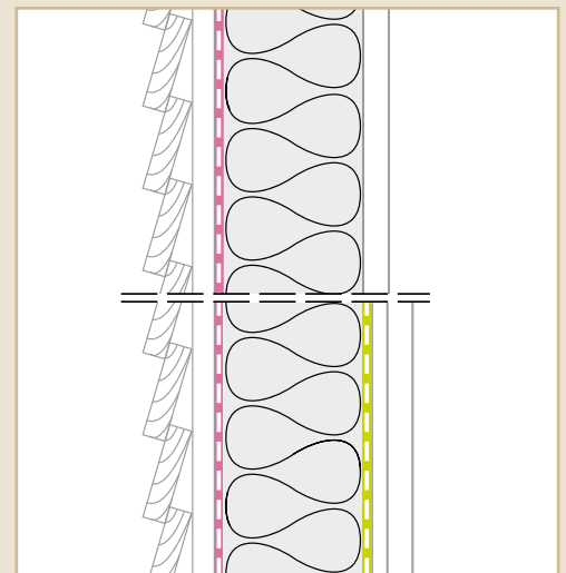
External wall wrap 0.75 MNs/g (low vapour resistance)
