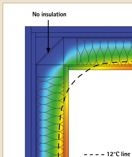
Uninsulated corners cause thermal bridges.
