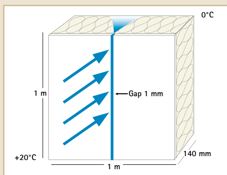
Fig. 16. Amount of moisture due to convection
